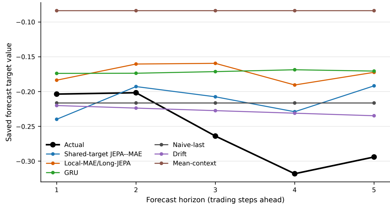
Representative forecast trajectory: NVDA, seed 42
