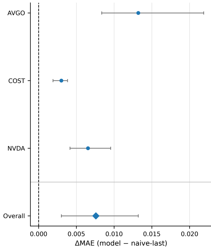
Shared-target JEP--MAE
