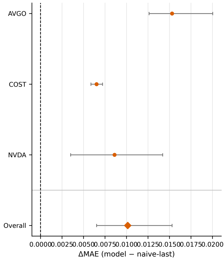
Local-MAE/Long-JEPA
