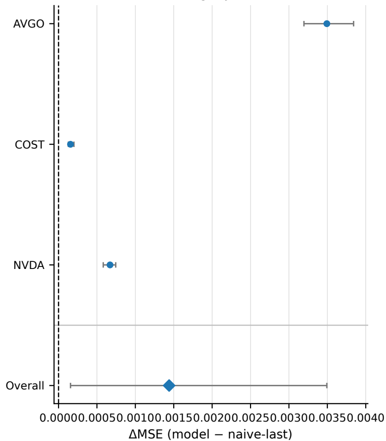
Shared-target JEPA--MAE
