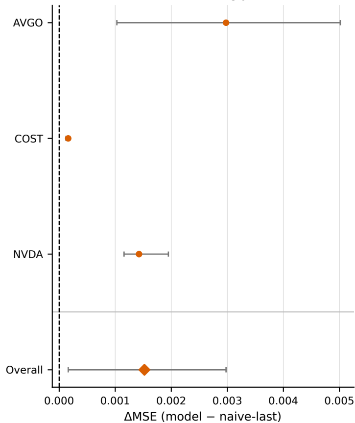
Local-MAE/Long-JEPA
