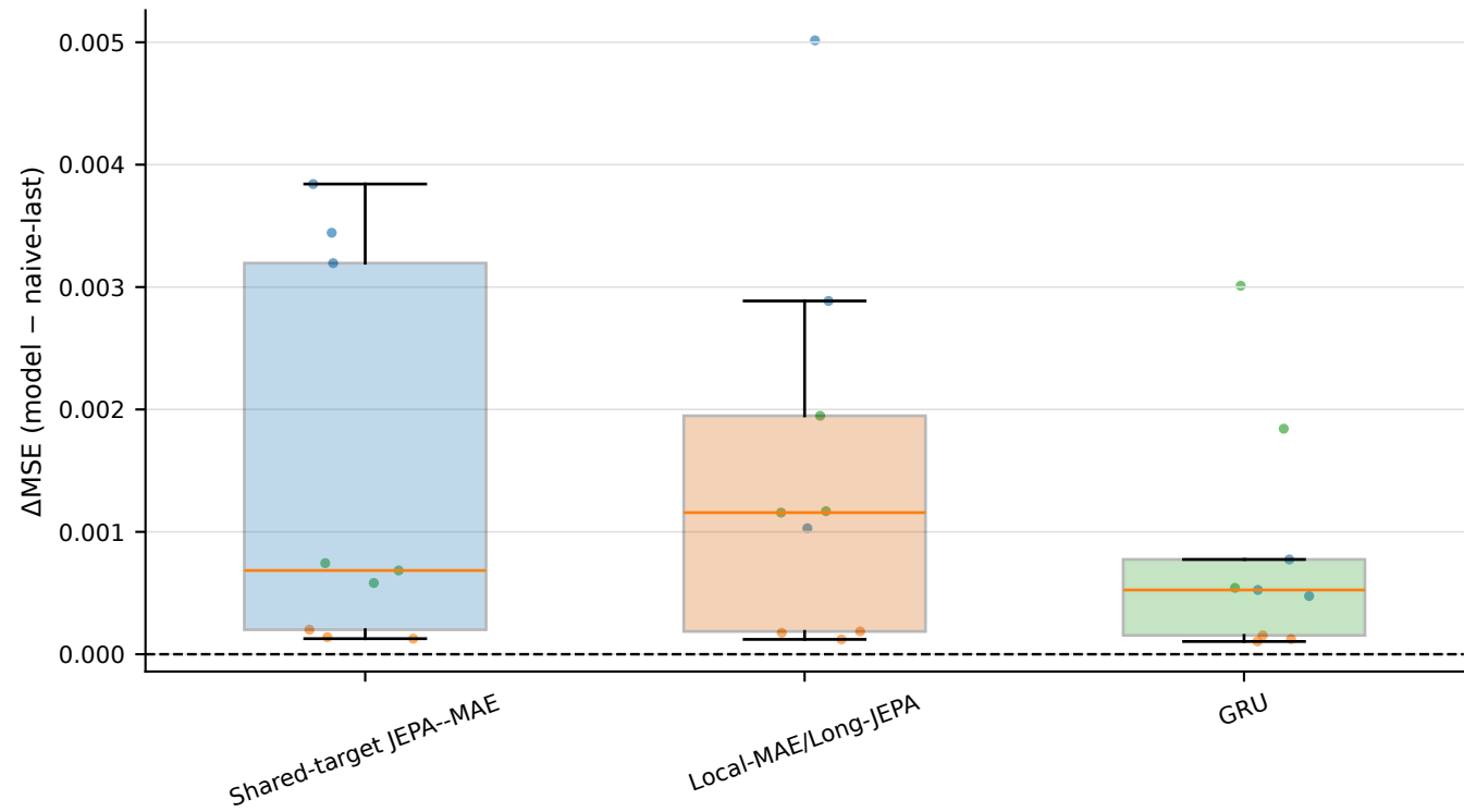
Seed-level paired MSE differences (descriptive)
