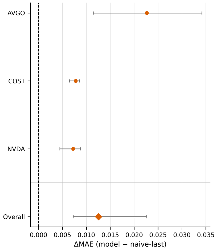
Local-MAE/Long-JEPA
