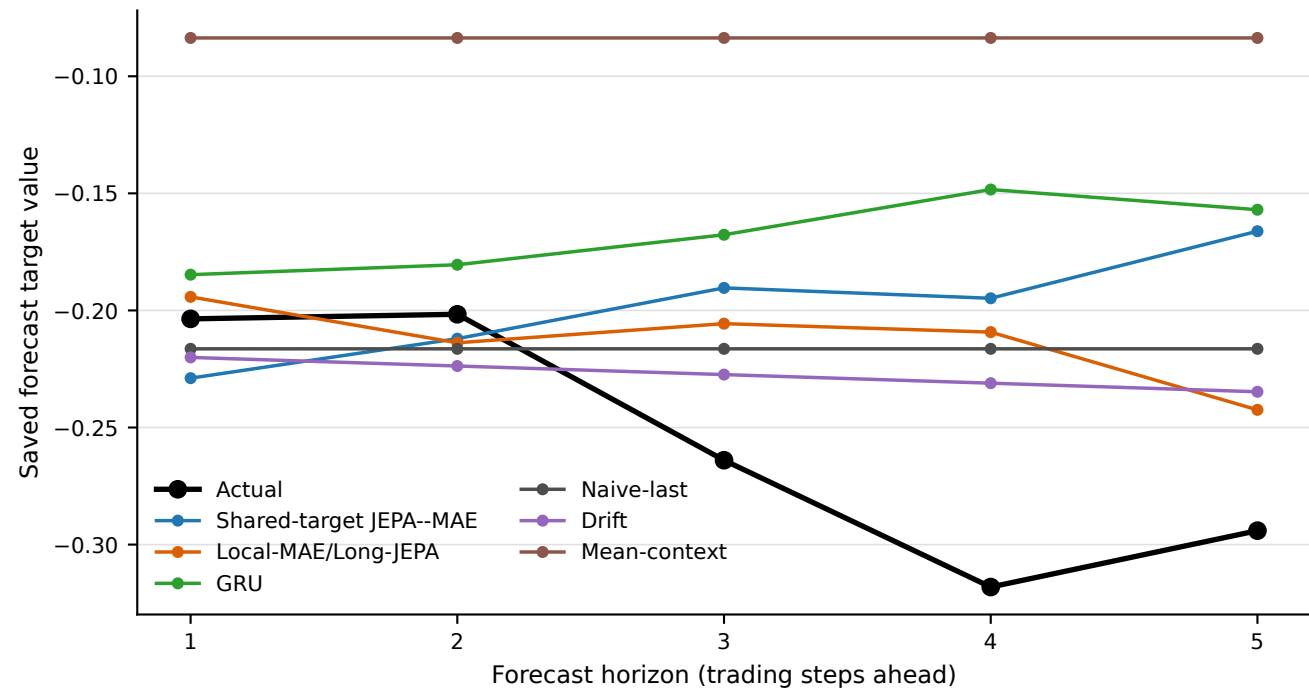
Representative forecast trajectory: NVDA, seed 46
