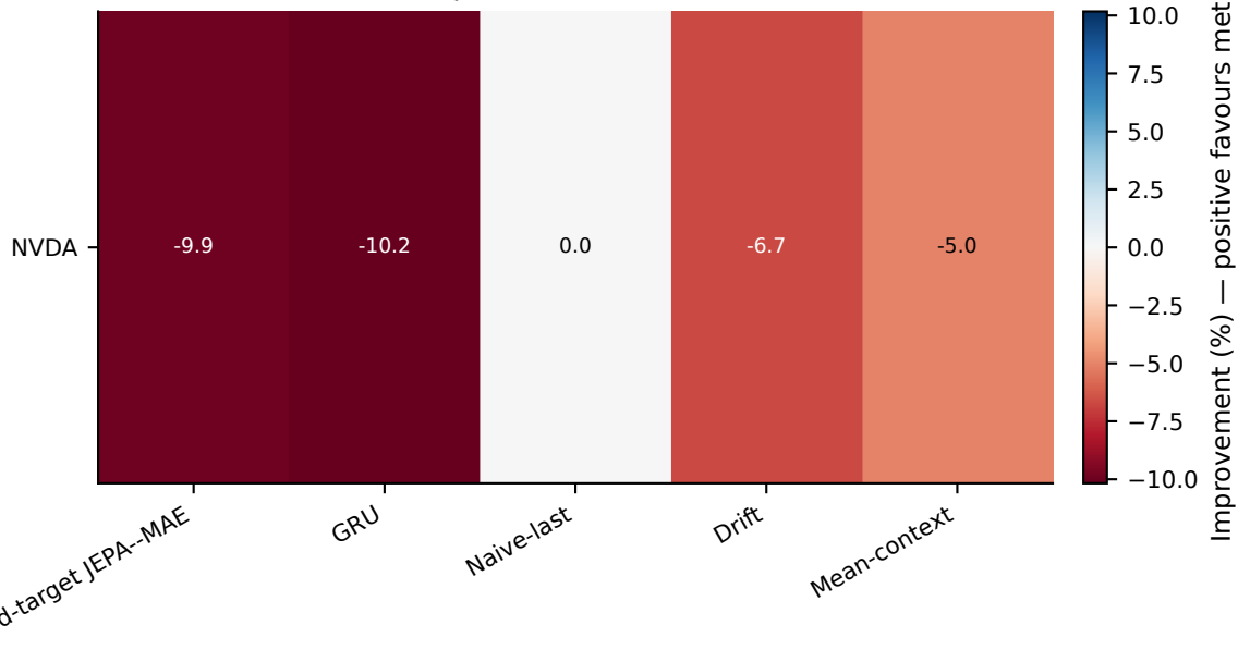
Relative MSE performance versus naive-last
