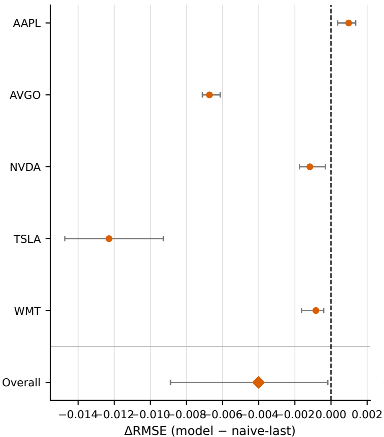
Local-MAE/Long-JEPA
