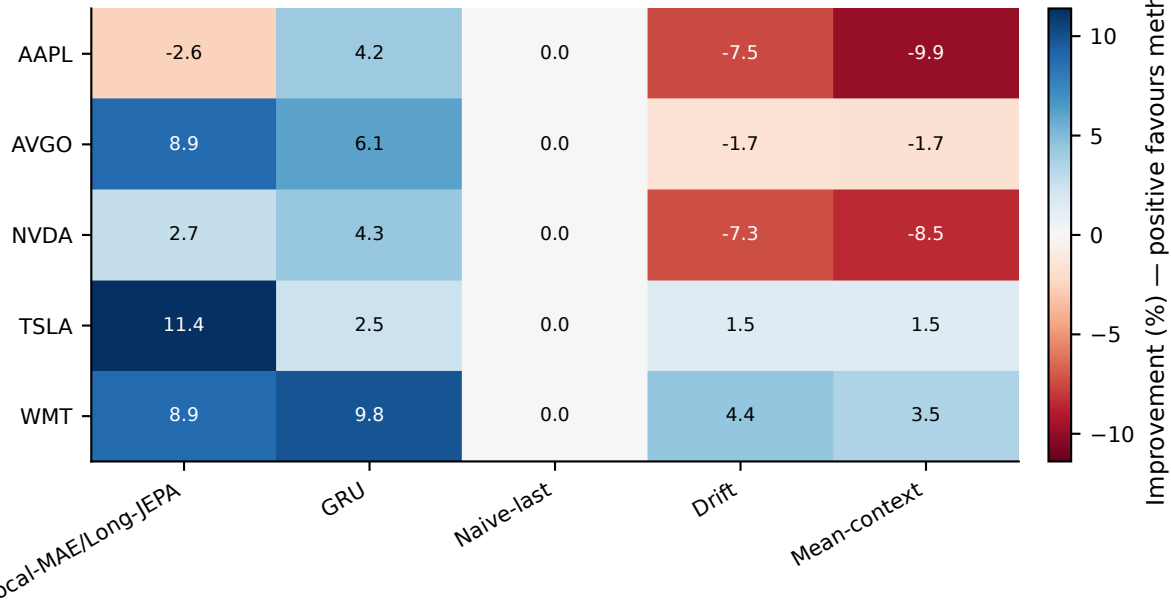
Relative RMSE performance versus naive-last
