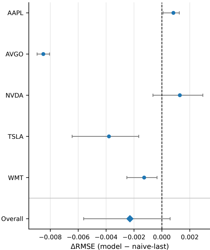
Shared-target JEPa--MAE
