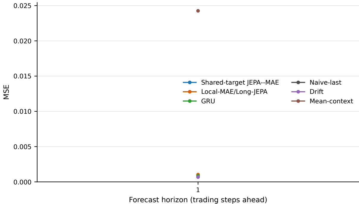
MSE by forecast horizon
