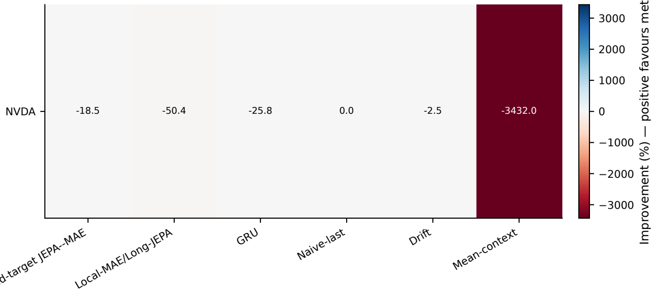
Relative MSE performance versus naive-last
