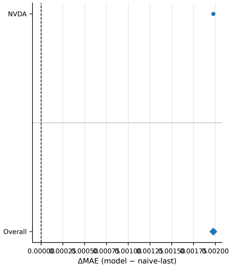
Shared-target JEPA--MAE
