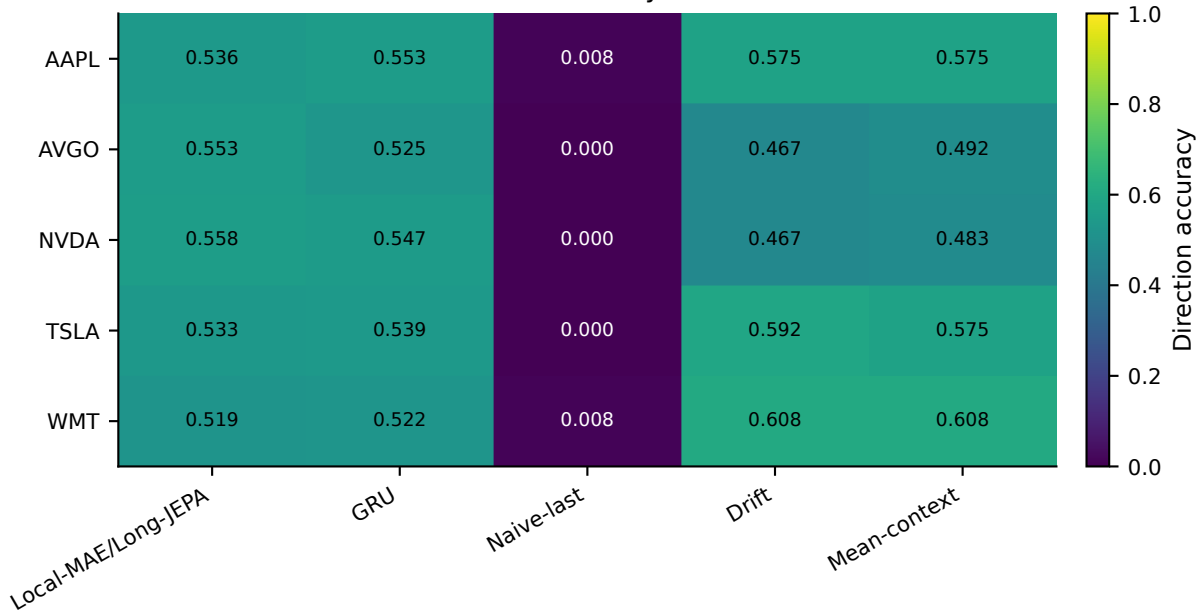
Mean direction accuracy across seeds
