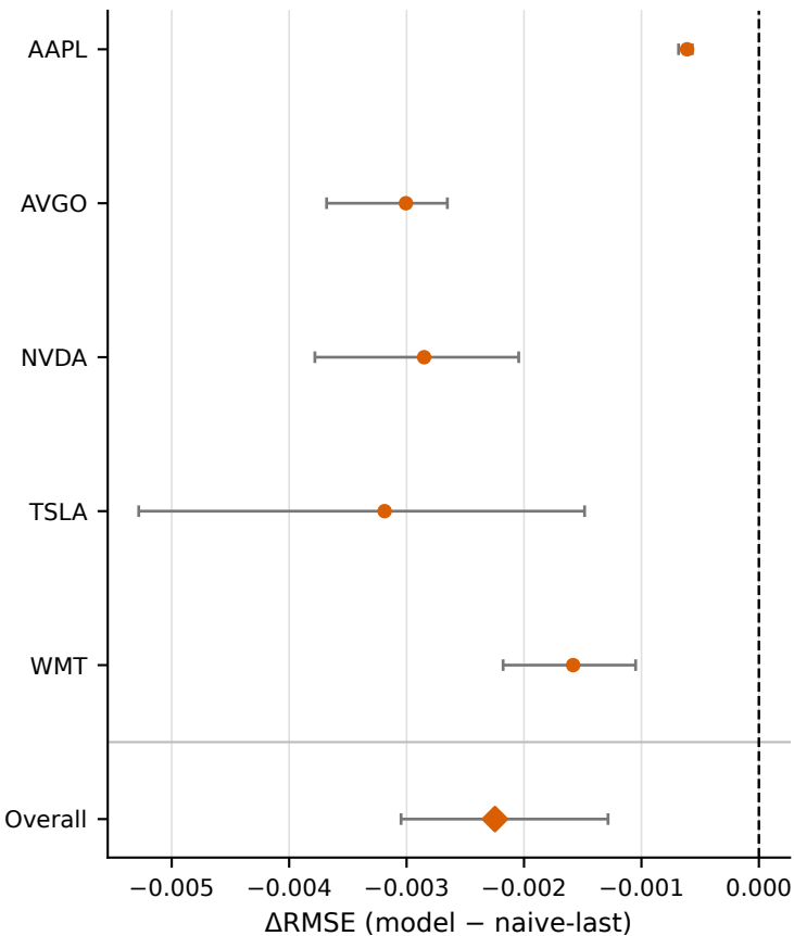
Local-MAE/Long-JEPA
