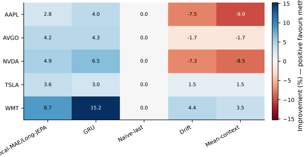
Relative RMSE performance versus naive-last
