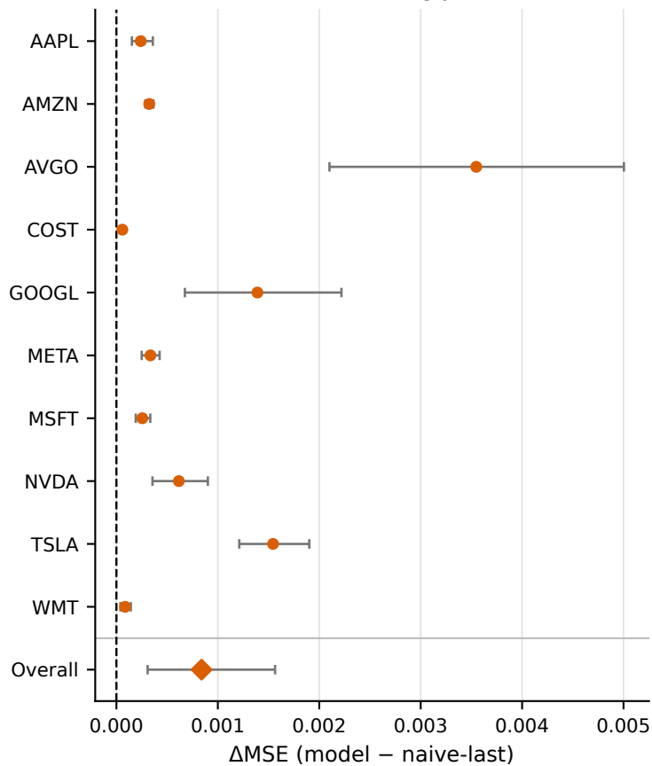
Local-MAE/Long-JEPa
