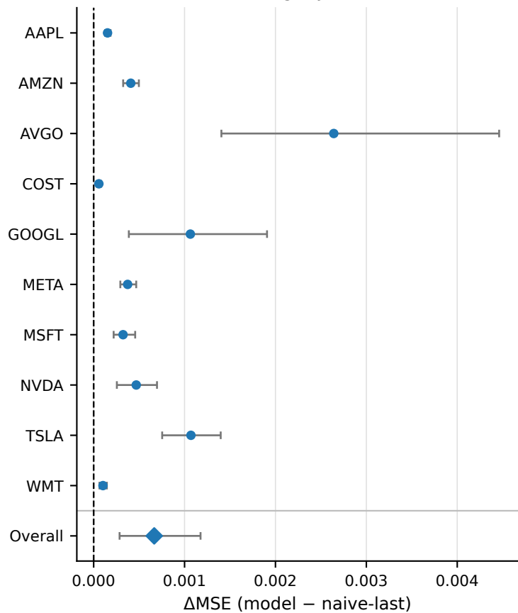
Shared-target JEPa--MAE
