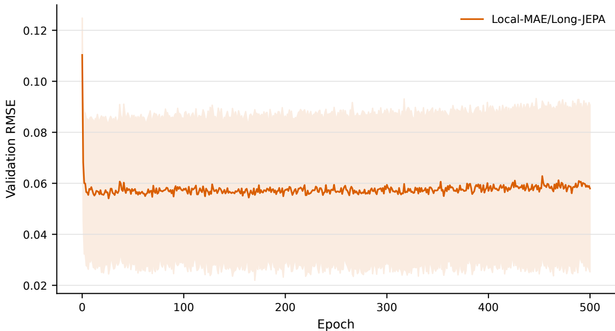
Validation RMSE (mean across stocks after seed averaging)
