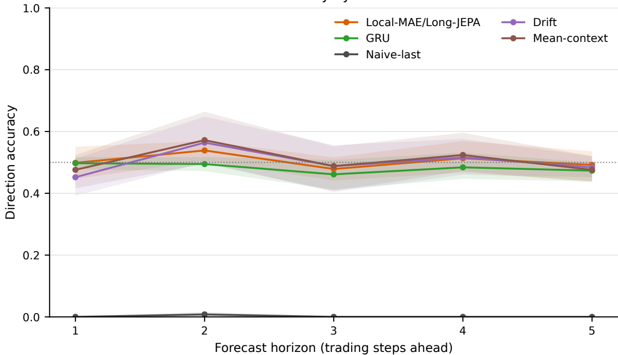
Direction accuracy by forecast horizon
