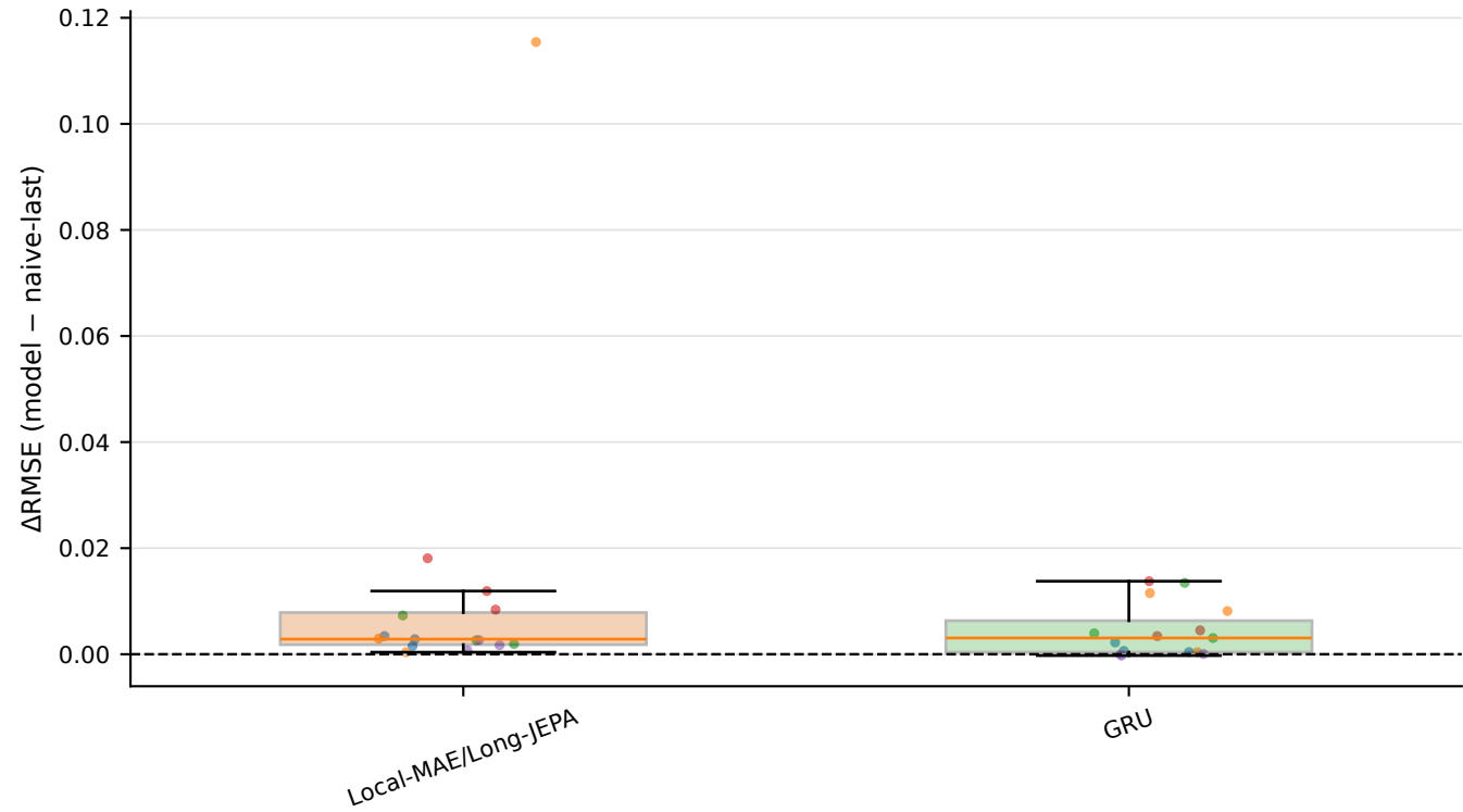
Seed-level paired RMSE differences (descriptive)
