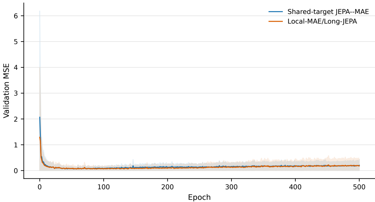
Validation MSE (mean across stocks after seed averaging)
