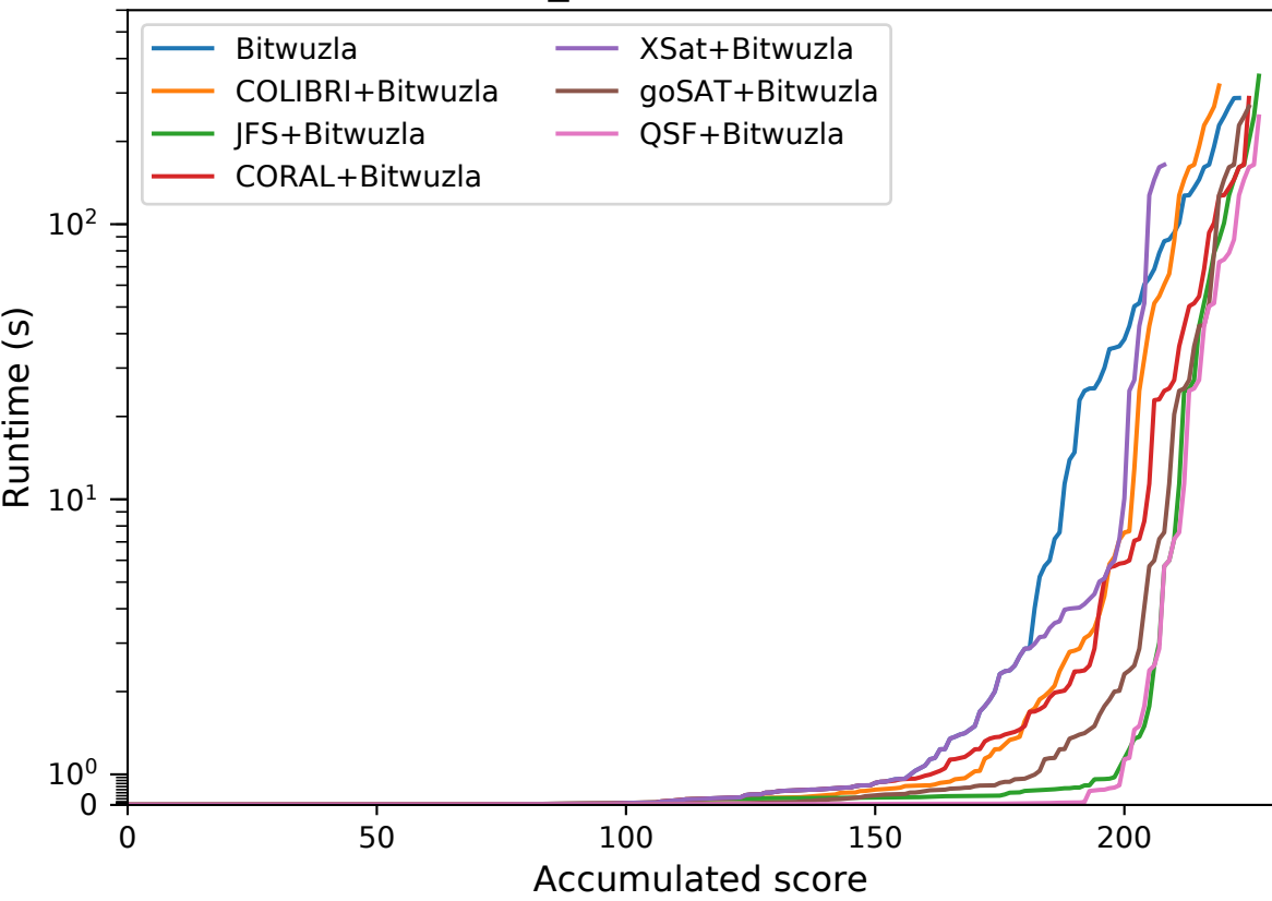
SMTLIB-QF_FP, 600 seconds timeout
