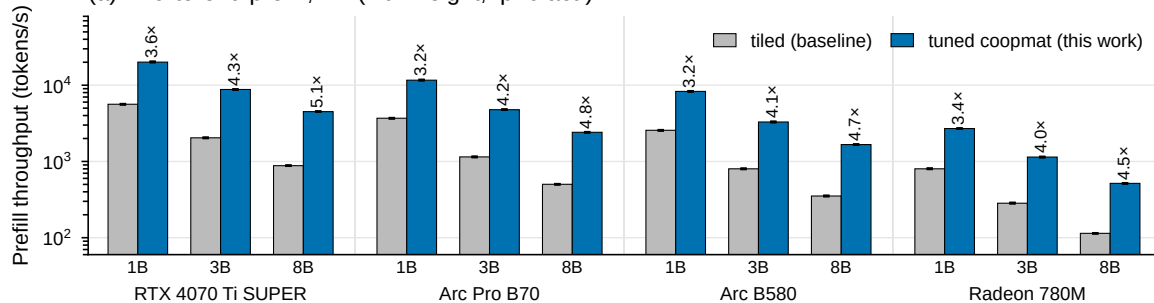
(a) End-to-end prefill, 4w (int4 weight, fp16 act.)
