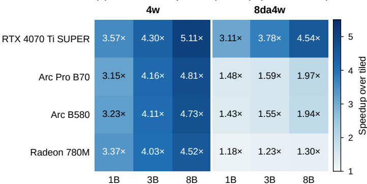
(c) End-to-end prefill speedup (tuned / tiled)
