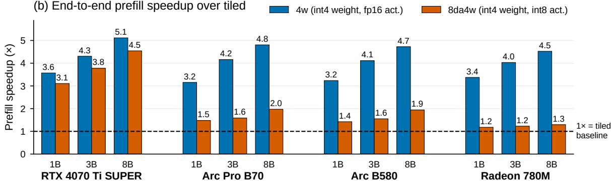
(b) End-to-end prefill speedup over tiled
