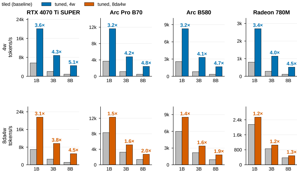
(a) End-to-end prefill throughput, 2048-token prompt (linear scale; each panel on its own axis)
