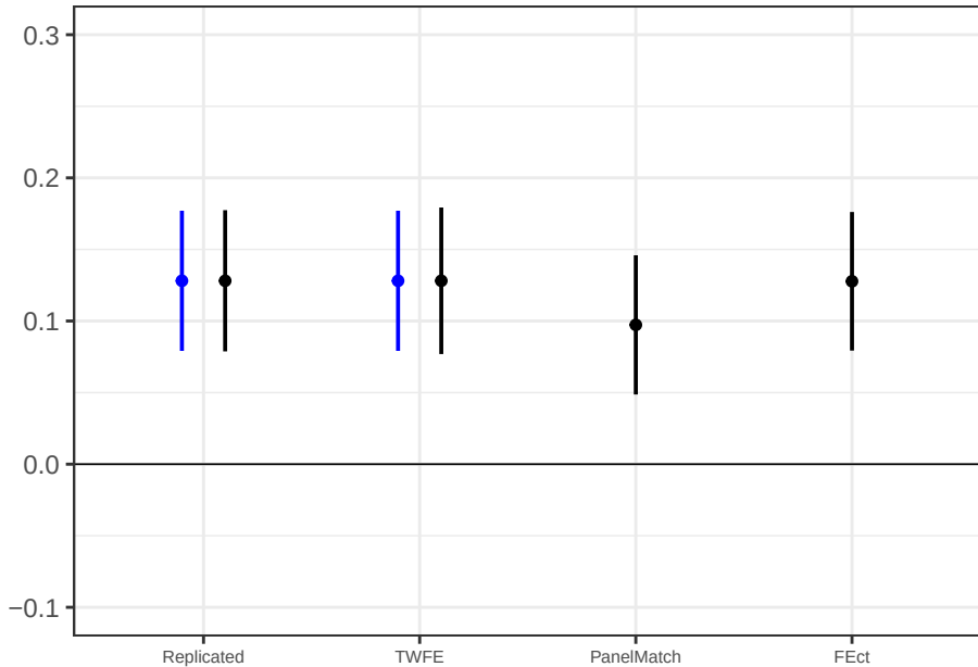
Coefficient and 95% CI
