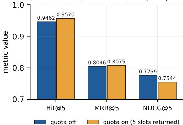
A. Metric levels with the source quota off vs on (conditional_93, both forms pooled, 186 pairs)
