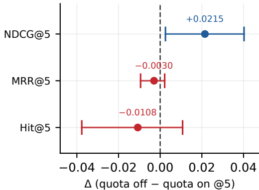
B. Paired bootstrap of the difference (2,000 resamples)
