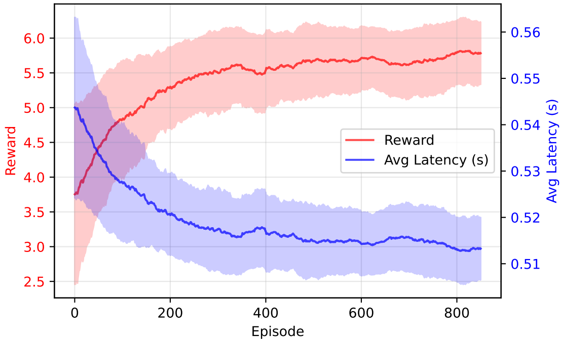
Convergence Analysis (Mean \pm Std over 5 seeds)
