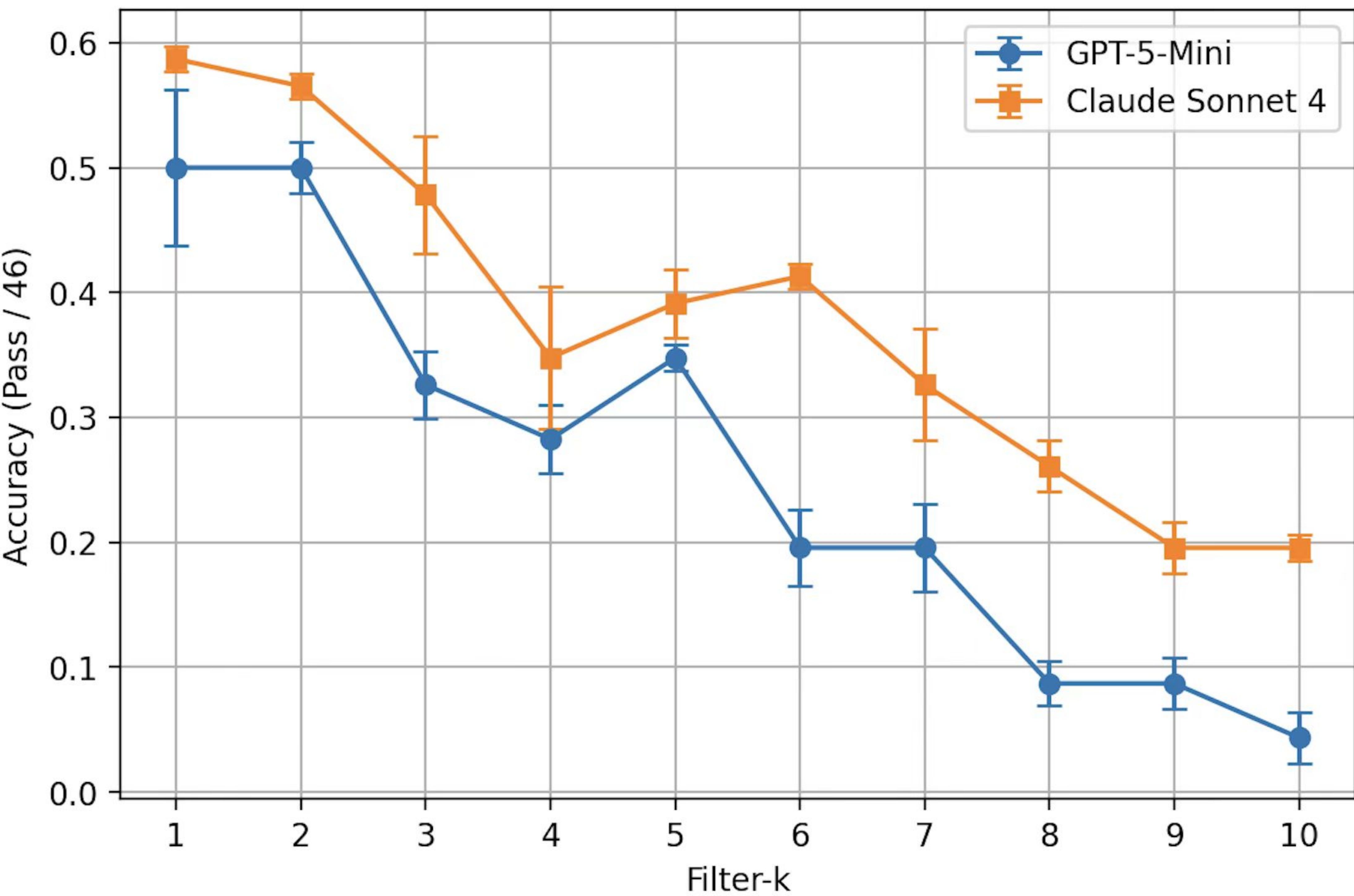
Accuracy vs Filter-k Median \pm Std across runs
