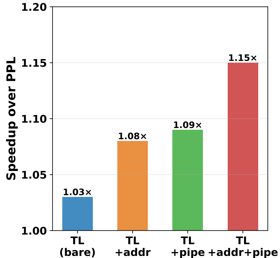
(b) Matmul
