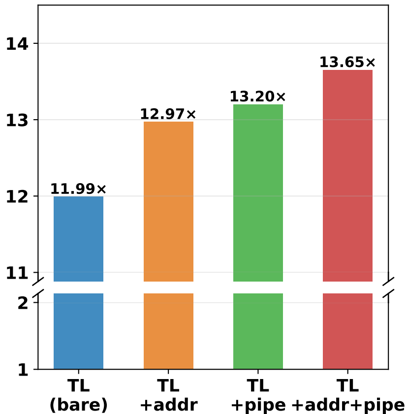
(a) FlashAttention
