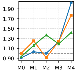
(e) RMSNorm
