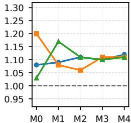
(c) SwiGLU
