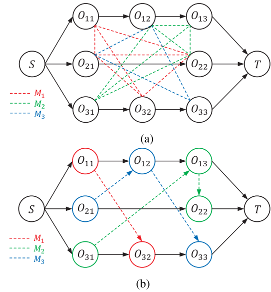
Fig. 1. Disjunctive graph for FJSP. (a) FJSP instance. (b) Possible solution.
