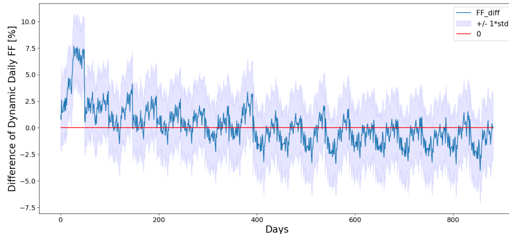
Figure 2: The improvement of the FF during the training. The graph shows the mean difference and standard deviation between the FF of the RL runs compared to their respective reference runs with the same random seed in percent. A negative value means improvement over the reference. After 50 days, the simulation is reset and a new episode is started with the same initial conditions.
