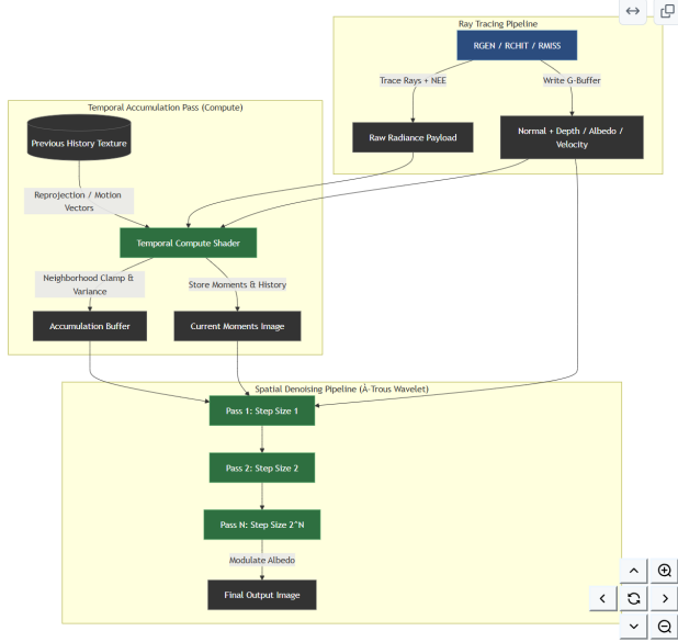
Figure 2: System architecture diagram depicting data flow across ray generation, temporal history integration, and multi-pass a-trous spatial filtering.
