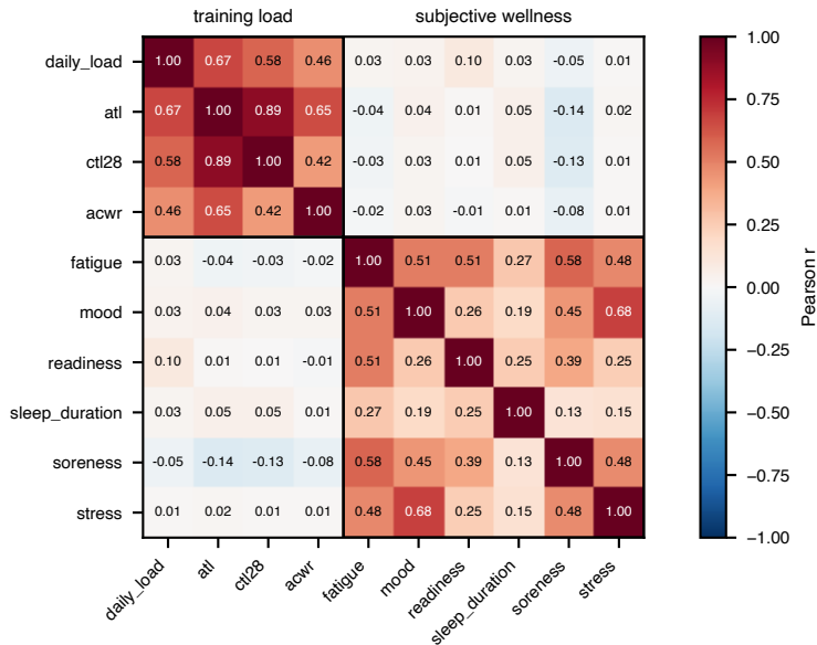
Inter-channel correlation, SoccerMon (35,550 windows \times 14 days)
