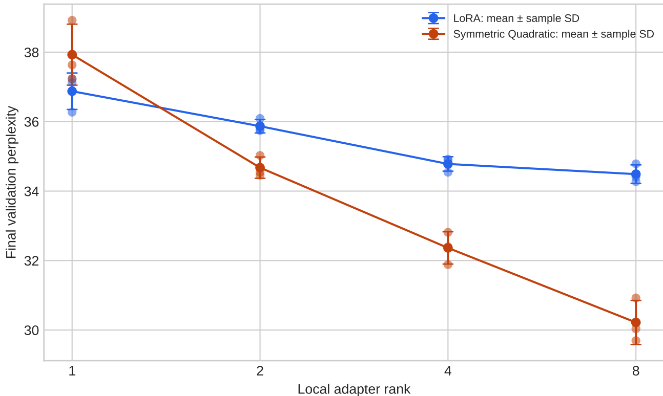
Controlled WikiText-2 rank screening: 1,000 steps, three seeds
