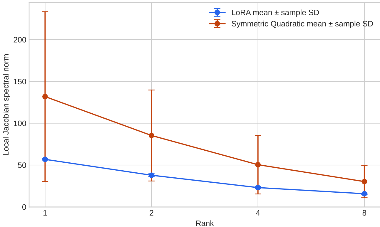
Fixed held-out WikiText-2 activation sample
