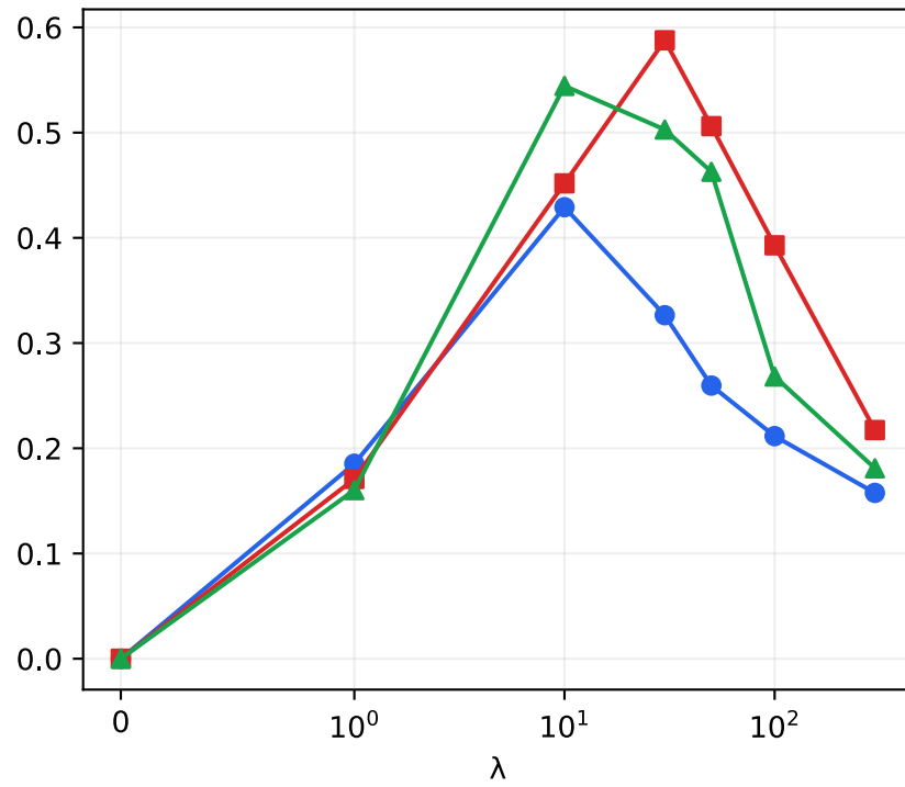
Realized EWC penalty C
