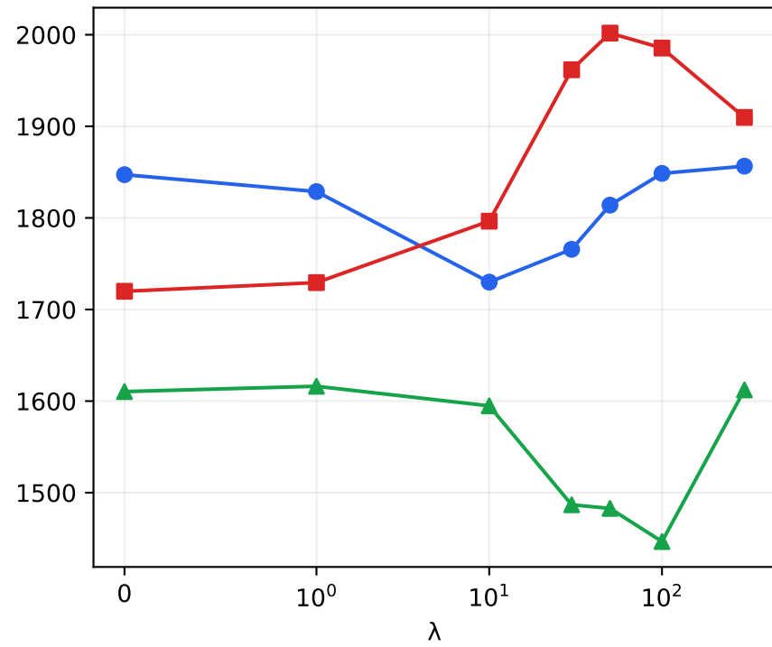
Fisher effective support
