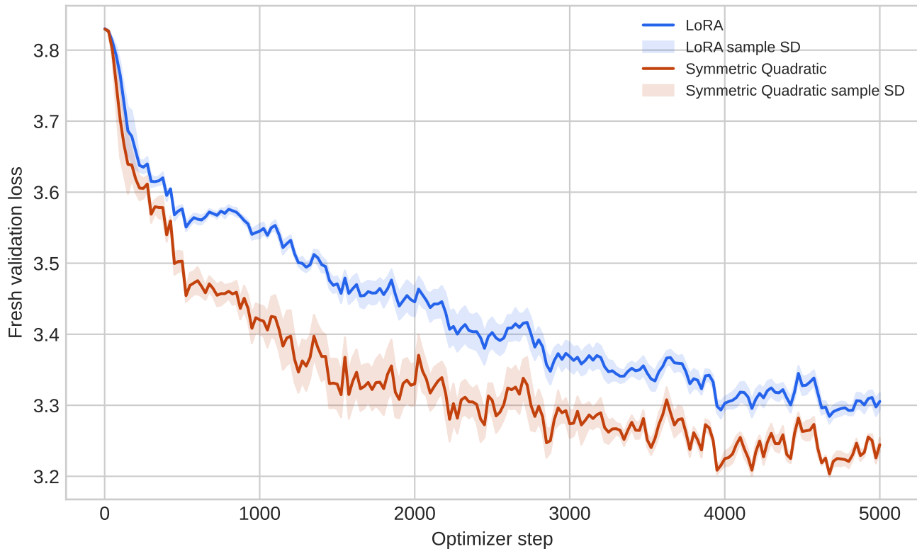
5,000-step convergence, rank 8
