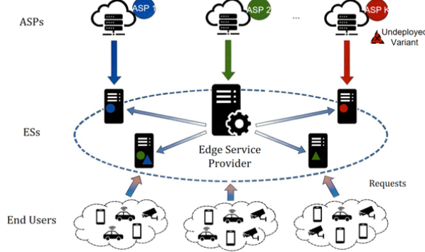
Fig. 1. System model: ASPs competitively place heterogeneous model variants on capacity-limited edge servers managed by the ESP.
