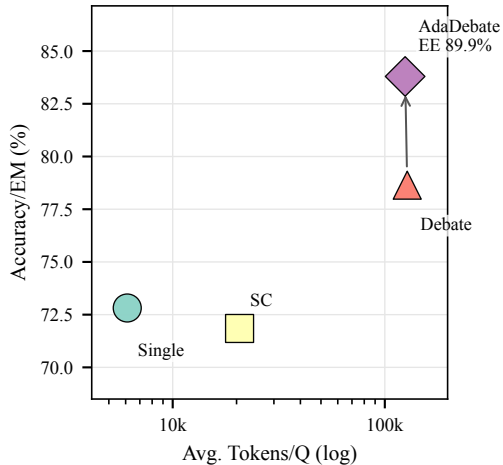
QuALITY (N=1043)
