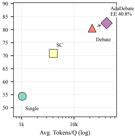
MMLU-Pro-Math (N=1351)
