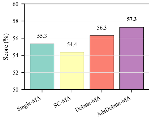
Exact Match
