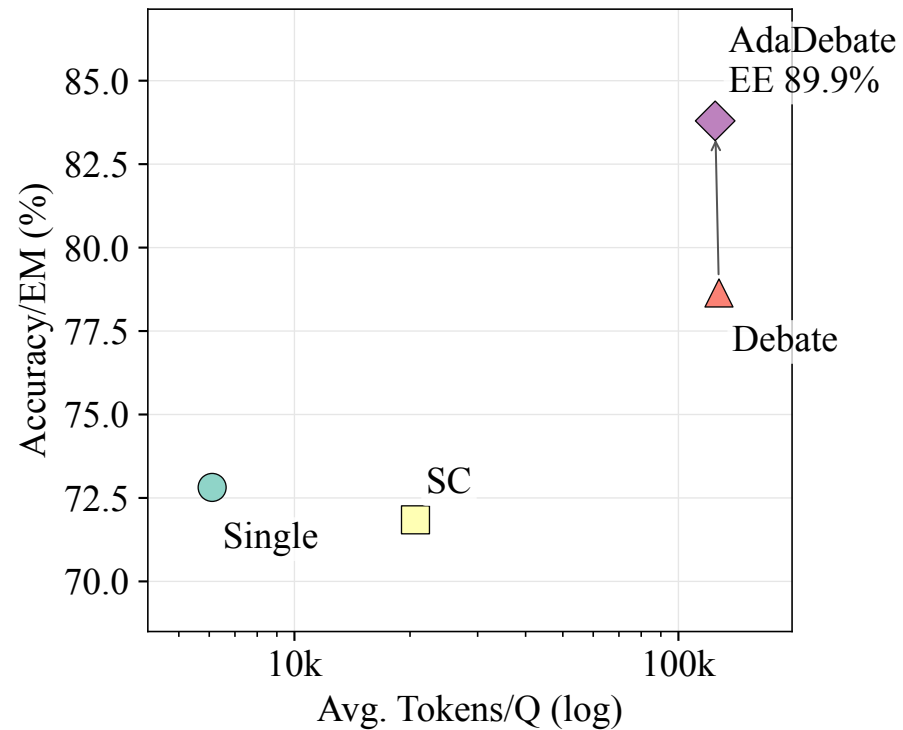
QuALITY (N=1043)
