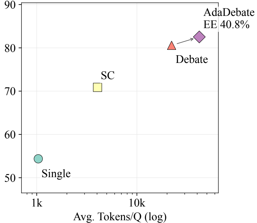
MMLU-Pro-Math (N=1351)
