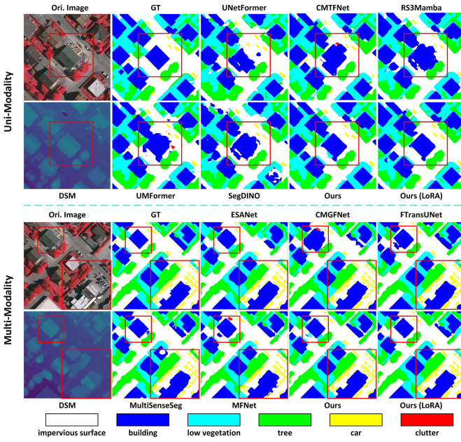
Fig. 5. Visualized comparisons on the Vaihingen test set. To highlight the differences, some red boxes are added to all subfigures. Specifically, the upper part of the figure presents the results of uni-modal methods, while the lower part shows those of multimodal methods.
