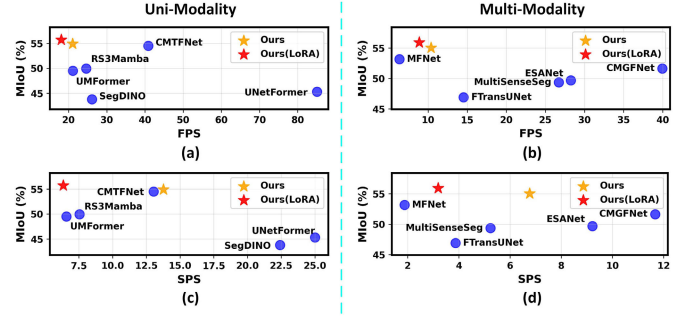
Fig. 9. Tradeoff between inference/training speed and segmentation accuracy on the WHU-OPT-SAR test set (on 256 \times 256 resolution images, batch size = 1). (a) Inference speed (FPS) versus mIoU on uni-modal tasks. (b) Inference speed (FPS) versus mIoU on multimodal tasks. (c) Training throughput (SPS) versus mIoU on uni-modal tasks. (d) Training throughput (SPS) versus mIoU on multimodal tasks. “FPS”: Frames Per Second. “SPS”: Steps Per Second.
