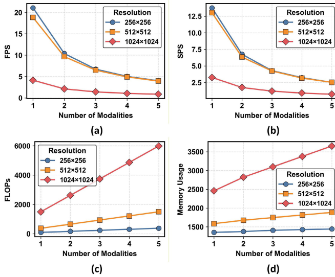
Fig. 10. Efficiency analysis of MM-DINO with DINOv3-L backbone under different input resolutions and varying numbers of modalities (batch size = 1). (a) Inference speed (FPS) versus number of modalities. (b) Training throughput (SPS) versus number of modalities. (c) FLOPs versus number of modalities. (d) GPU memory usage versus number of modalities. All metrics are measured on a single NVIDIA L20 GPU with 48-GB memory. The three curves in each subfigure correspond to input resolutions of 256 \times 256 , 512 \times 512 , and 1024 \times 1024 pixels, respectively.
