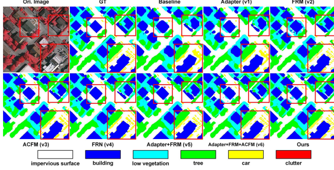
Fig. 8. Visual comparison of ablation studies on the Vaihingen test set. To highlight the differences, some red boxes are added to all subfigures.
