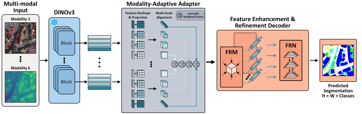
Fig. 2. Overview of the proposed MM-DINO framework for uni-modal and multimodal remote sensing image semantic segmentation. The architecture consists of three main components: 1) a frozen pretrained DINOv3 backbone that extracts multilevel visual features from input modalities; 2) a modality-adaptive adapter that reshapes, aligns, and performs early cross-modal interaction through learnable adaptive weights; and 3) a feature enhancement and refinement decoder composed of an FRM, an ACFM, and an FRN for multiscale fusion and upsampling to produce the final segmentation map. The framework supports both single-modal (e.g., RGB only) and multimodal (e.g., RGB + DSM) inputs, as illustrated by the separate modality paths that converge at the adapter stage. Arrows indicate the flow of features through the network.
