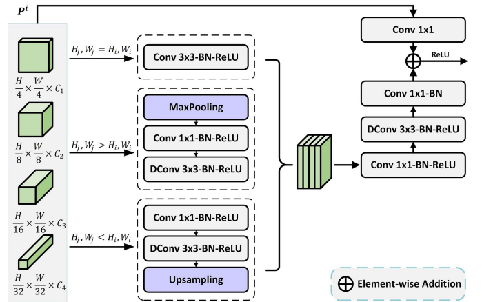
Fig. 3. Structure of the FRM. This module enriches the contextual representation of each input feature scale by generating multireceptive-field contextual features through parallel convolutional branches. The aligned outputs from all branches are concatenated and then fused with the original inputs via a lightweight residual fusion block, producing enhanced features that preserve fine details while integrating rich context.
