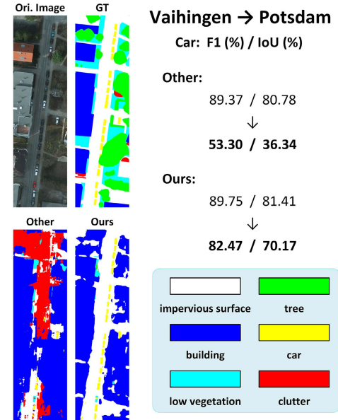
Fig. 1. Cross-dataset generalization results (trained on Vaihingen and tested on Potsdam). Visualized comparisons are provided to intuitively show the segmentation performance of uni-modal and multimodal methods on the Potsdam test set.
