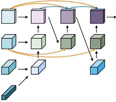
Fig. 4. Structure of the FRN. This module adopts a strategy combining top-down and iterative refinement. First, high-level semantic features are upsampled and fused with lower level detailed features step by step (top-down pathway). Then, local iterative units are introduced at key levels, progressively enhancing the semantic consistency and boundary accuracy of features by repeatedly fusing the current features, the refined output from the previous step, and the original backbone features.
