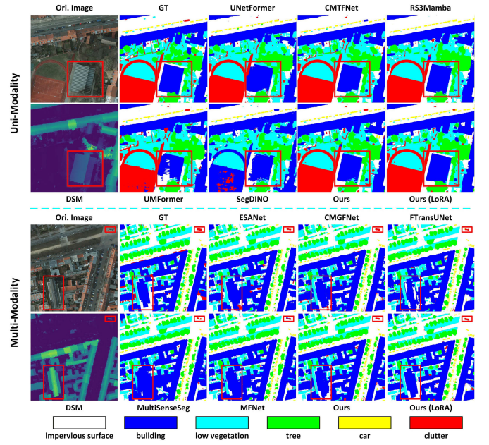
Fig. 6. Visualized comparisons on the Potsdam test set. To highlight the differences, some red boxes are added to all subfigures. Specifically, the upper part of the figure presents the results of uni-modal methods, while the lower part shows those of multimodal methods.
