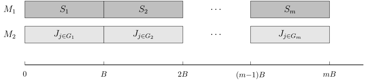
Figure 3-2: 3-Partition reduction schedule.
