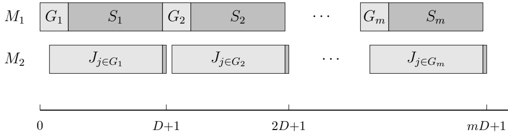
Figure 3-2: 3-Partition reduction
