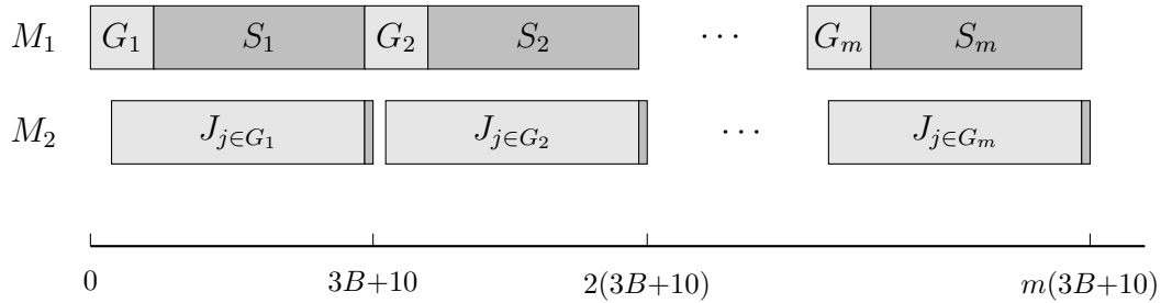
Figure 3-2: 3-Partition reduction (scaled by 3)
