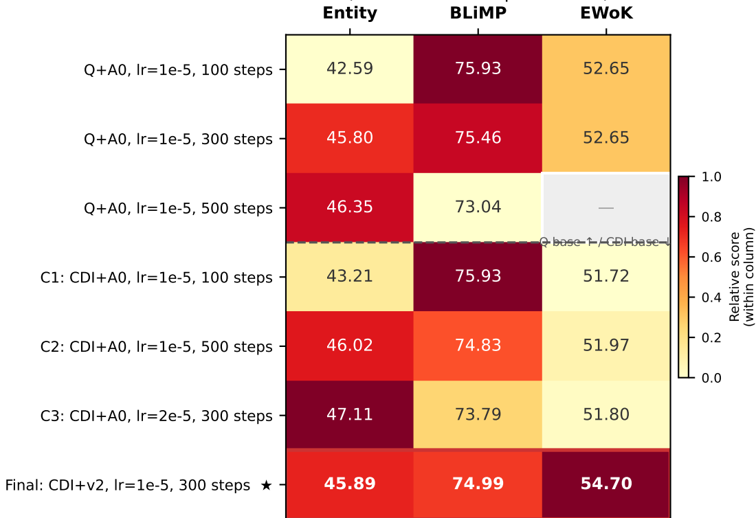
SimPER Hyperparameter Sensitivity (color normalized per column)
