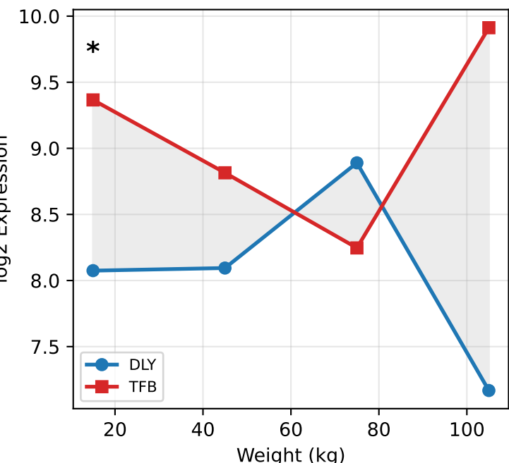
CPS1
