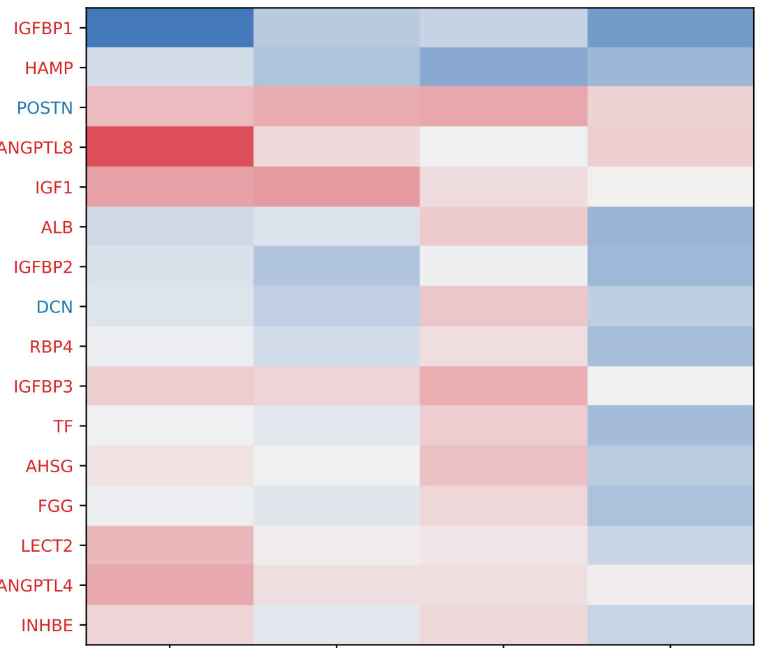
Liver: Hepatokine/Myokine log2FC (DLY vs TFB)
