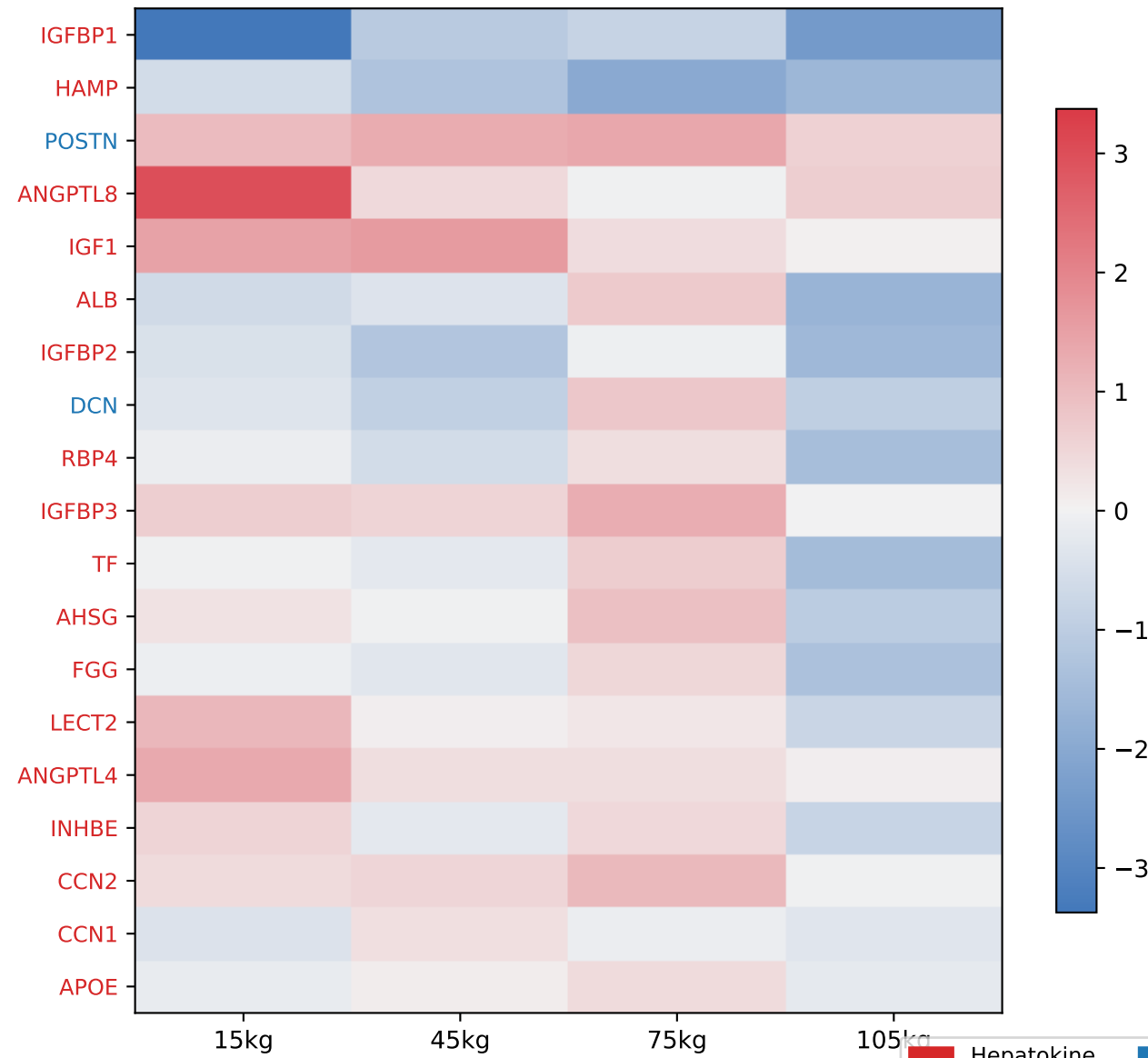
Liver: Hepatokine/Myokine log2FC (DLY vs TFB)
