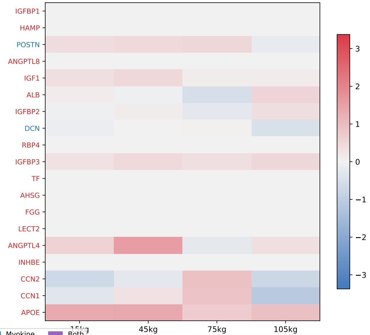
Muscle: Corresponding log2FC (Full 24784-gene matrix)
